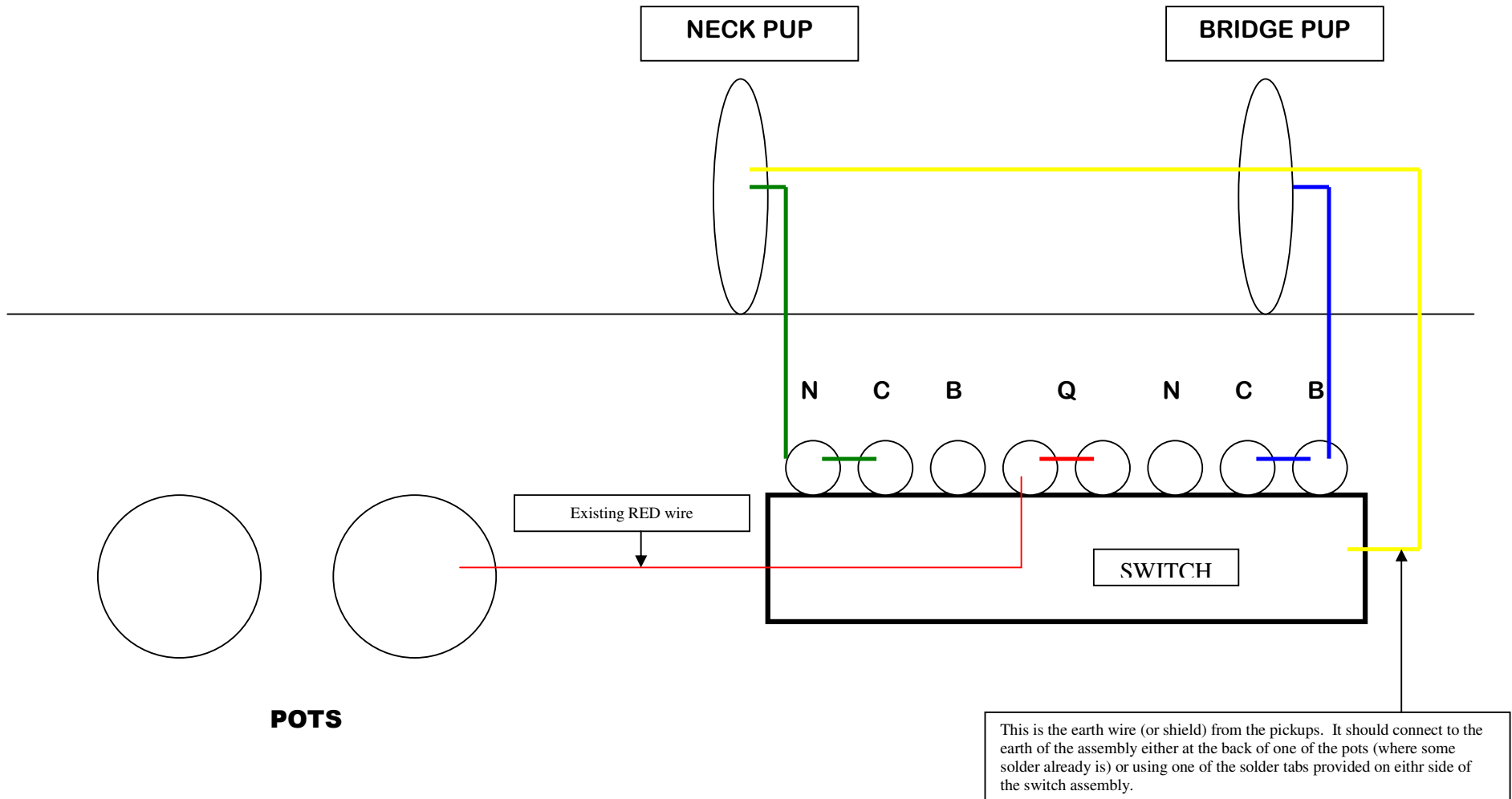
View From Rear of Tele Control Assembly
